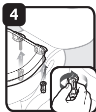
Attach nuts and finger-tighten, keeping washer aligned with the hinge body
