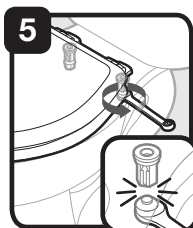
As you hold seat centered on bowl, tighten lower section of STA-TITE® nuts until they snap off
