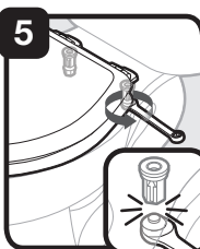
As you hold seat centered on bowl, tighten lower section of STA-TITE® nuts until they snap off
