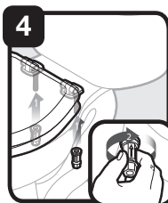
Attach nuts and finger-tighten, keeping washer aligned with the hinge body
